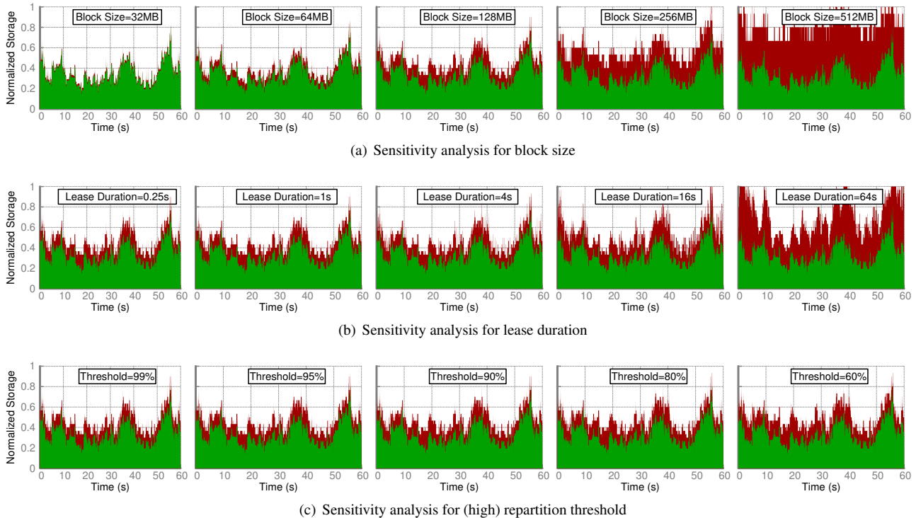
Fig. 14. Jiffy sensitivity analysis for (a) block size (b) lease duration and (c) repartition threshold for the file data structure. Green area corresponds to used capacity, while red area corresponds to allocated capacity under Jiffy. See §6.6 for details.
