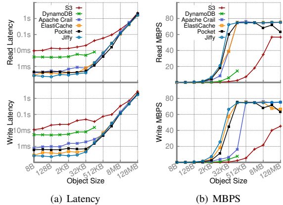
Fig. 10. Jiffy performance comparison with existing systems (§6.2). Despite providing the additional benefits demonstrated in §6.1, Jiffy performs as well as state-of-the-art systems commonly used for intermediate data storage in serverless analytics.
