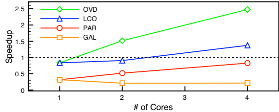
Figure 7. Speedup vs. # of cores for B-K maxflow
