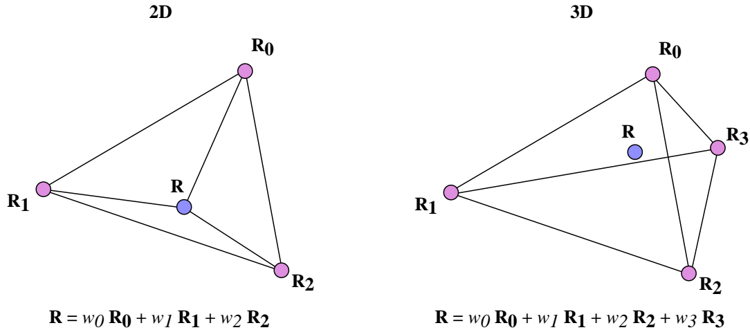
Figure 3-13: A simplex in 2D and 3D: triangle and tetrahedron.
