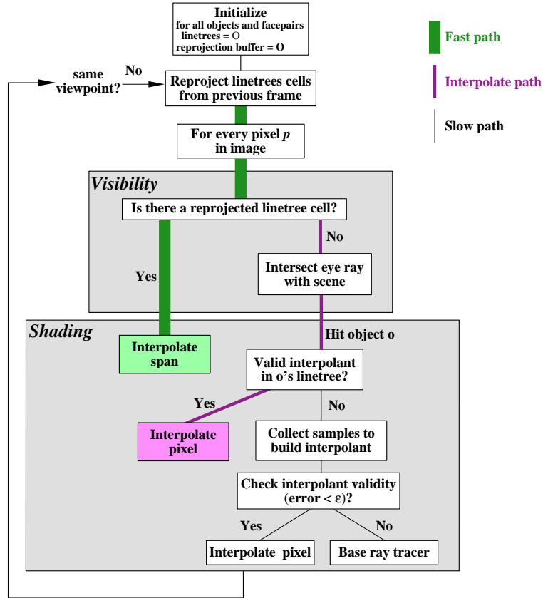
Fig. 1. Algorithm Overview.
