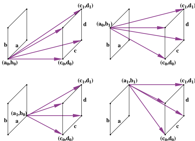
Fig. 7. 4D linetree cell and its sixteen extremal rays.
