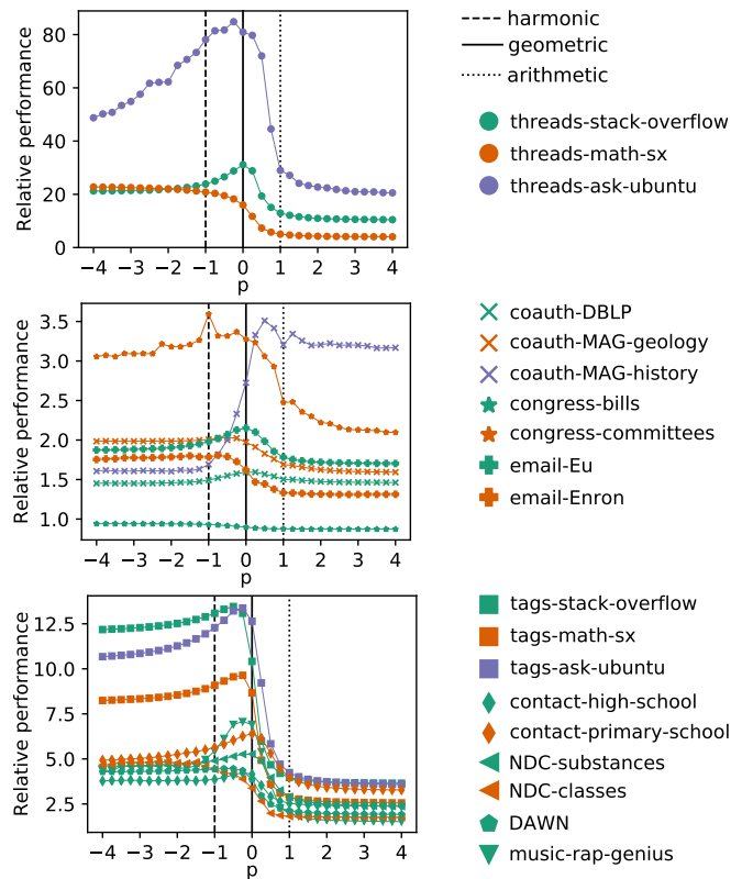
Fig. 7. AUC-PR relative to random predictions as a function of the parameter p in the generalized mean heuristic model for higher-order link prediction.
