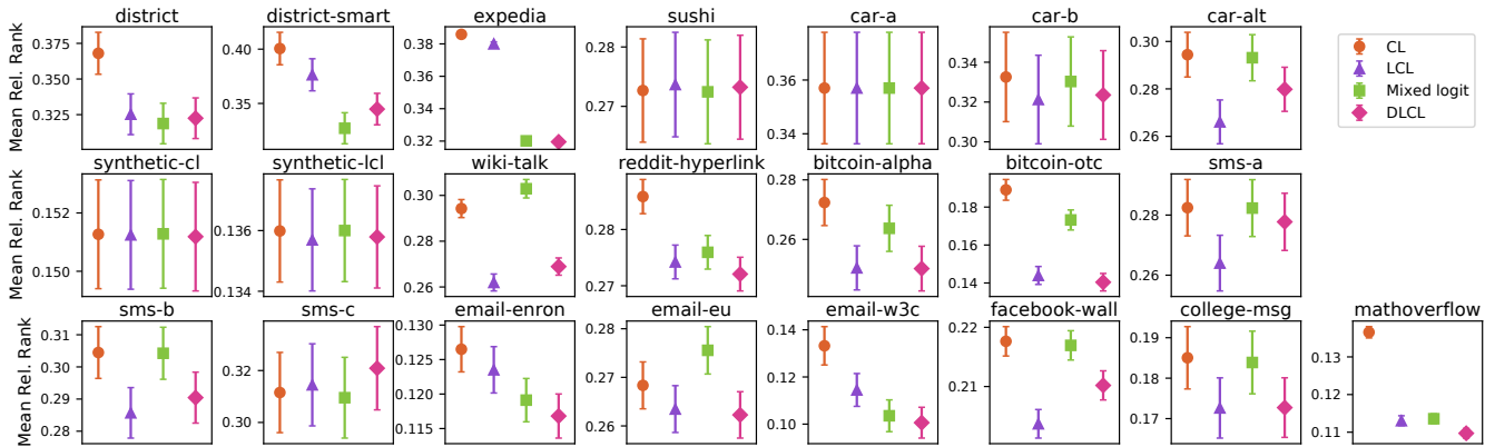
Figure 2: Mean relative rank of predictions on held-out test data (lower is better). Error bars show standard error of the mean.
