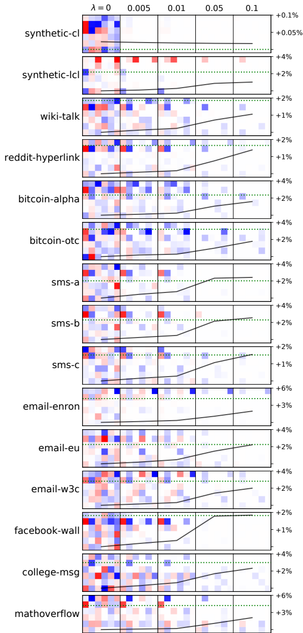
Figure 3: Effect of L_1 regularization on the LCL context effect matrix. The parameter \lambda (increasing left to right) controls the strength of regularization. Each box visualizes the learned matrix A (blue = negative, red = positive, white = zero; consistent color scales within but not between rows) at the given \lambda value. Features in A are in the order from Section 6.2, top-down and left-right. The black line tracks the total NLL of the LCL (the % on the y-axes is relative to the NLL of the best model plotted for that dataset). The dotted green line is the significance threshold of a likelihood-ratio test against a CL ( p < 0.001 ; black line below the threshold means the LCL is a significantly better fit than CL).
