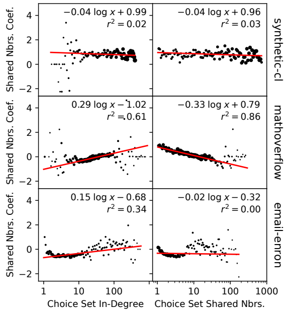
Figure 1: Learned preference coefficients of CLs trained on samples binned by mean choice set feature. Each point shows the preference coefficient of the shared neighbors feature in choice sets with varying mean in-degree (left column) and shared neighbor counts (right column). These coefficients were found by splitting observations into 100 bins according to their mean feature values and learning a CL for each bin separately. The area of each point is proportional to the square root of the number of observations in its bin. The red lines are weighted least squares fits.
