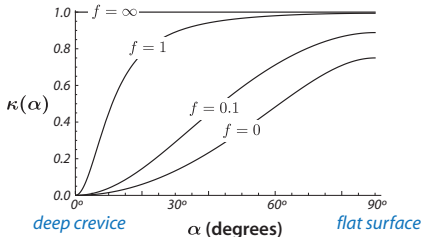
Figure 4. \kappa(\alpha) for different ratios of ambient to direct light f . Note that as f \rightarrow \infty ( l_d = 0 ) we have a constant curve ( \kappa(\alpha) = 1 ) so information about \alpha cannot be recovered.
