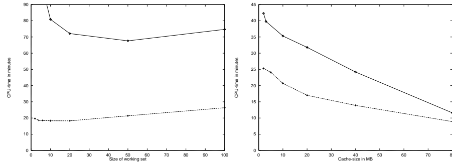
Figure 11.2 Training time dependent on working set size and cache size for the Ohsumed task.
