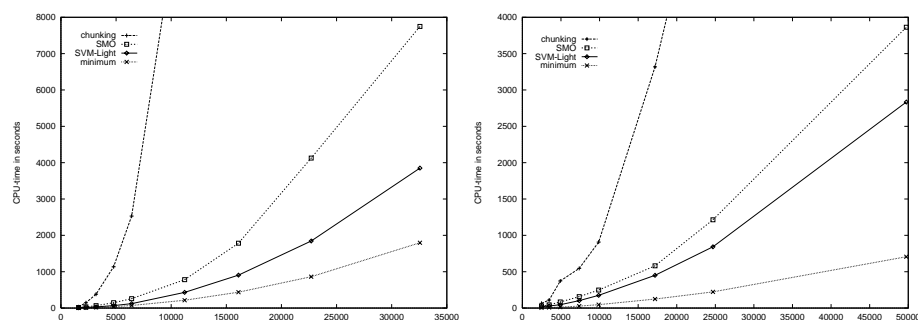
Figure 11.1 Training times from tables 11.1 (left) and 11.2 (right) as graphs.
