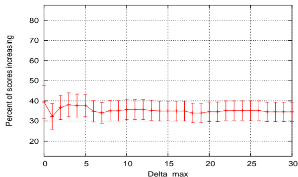
Figure 6: Percentage of swaps that increase performance vs. \delta_{max} for Physics.
