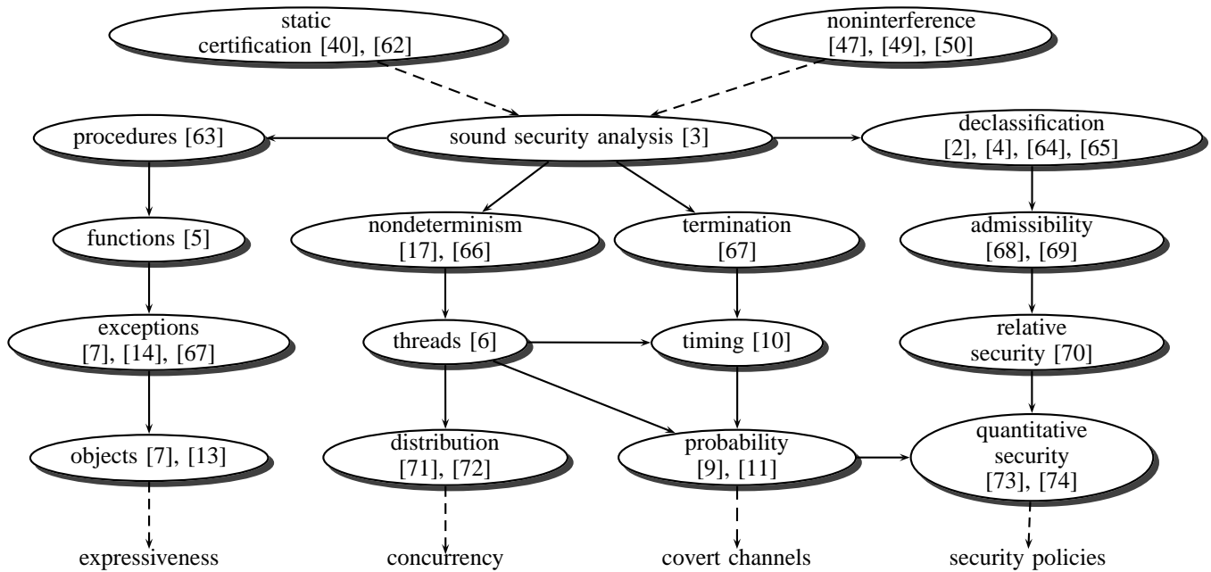
Fig. 4. Evolution of language-based information flow.
