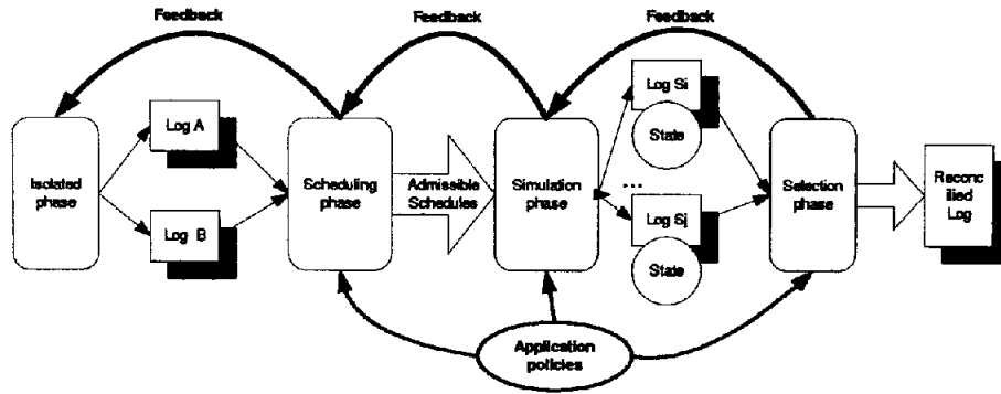
Figure 1: IceCube overview
